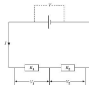
Figure 20.19 The potential divider
