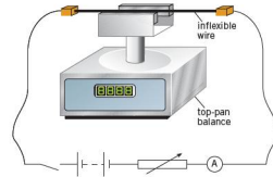
Figure 22.11 Apparatus to investigate the magnitude of the electromagnetic force
