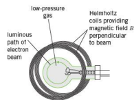
Figure 22.18 Fine-beam tube
