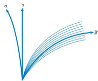
Figure 26.3 Deflection of \alpha - and \beta -particles and \gamma -radiation by a magnetic field into the page
