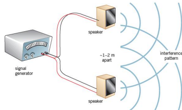
Figure 15.7 Demonstration of interference with sound waves
