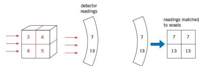
Figure 25.34 The first set of detector readings
