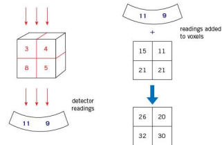
Figure 25.36 The third set of detector readings
