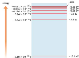
Figure 25.9 Electron energy levels for the hydrogen atom
