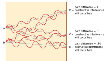
Figure 15.6 Producing an interference pattern
