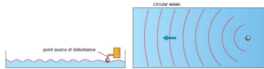
Figure 14.8 Ripple tank pattern for a point source
