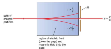
Figure 22.22 Velocity selector
