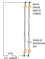
Figure 22.13 Apparatus to demonstrate the force between parallel current-carrying conductors
