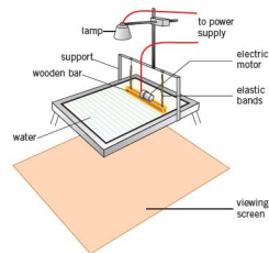
Figure 14.6 Ripple tank
