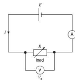
Figure 20.4 Circuit for investigating power transfer to an external load
