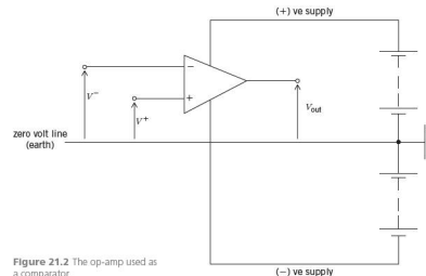
Figure 21.2 The op-amp used as a comparator
