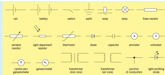
Figure 20.1 Circuit symbols
