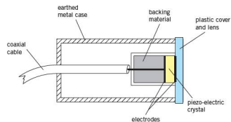
Figure 14.4 Piezo-electric transducer/receiver
