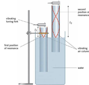
Figure 15.27 Speed of sound by the resonance tube method
