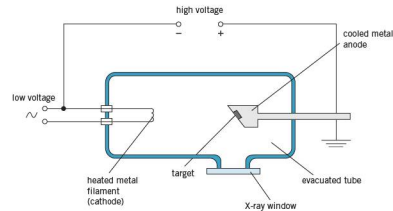
Figure 25.20 Design of an X-ray tube
