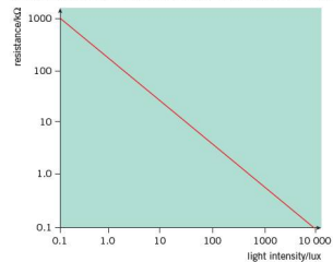
Figure 19.3 Resistance v. light intensity for an LDR
