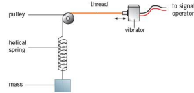
Figure 13.16 Demonstration of forced oscillations
