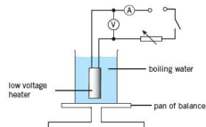
Figure 12.9 Apparatus to determine the latent heat of vaporisation of water
