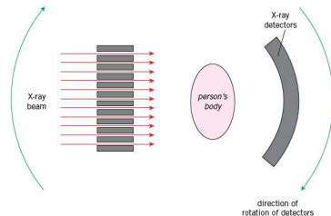
Figure 25.32 Arrangement for a CT scan
