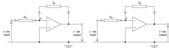
Figure 21.8 Feedback current
