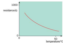
Figure 25.16 Change of resistance with temperature of a sample of an intrinsic semiconductor
