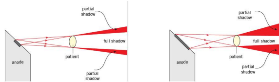
Figure 25.24 Effect of changing the area of the target anode on sharpness
