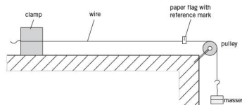
Figure 9.5 Simple experiment to measure the Young modulus of a wire
