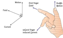
Figure 23.4 Fleming's right-hand rule
