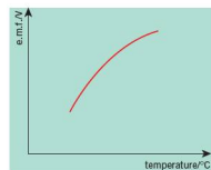
Figure 2.31 Calibration curve for a thermocouple
