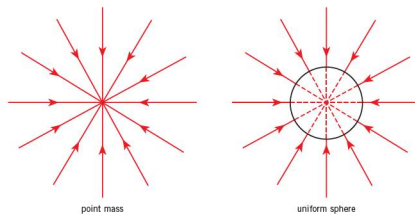
Figure 8.1 Gravitational fields
