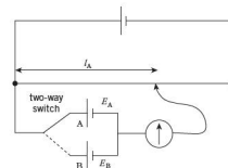
Figure 20.22 Potentiometer used to compare cell e.m.f.s
