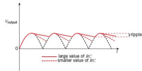
Figure 24.9 Magnitude of the ripple
