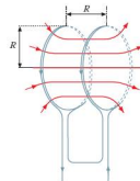
Figure 22.30 Magnetic field in Helmholtz coils
