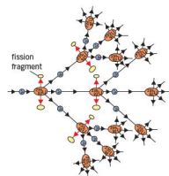
Figure 26.4 Accelerating chain reaction
