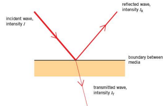
Figure 14.5 The reflection and transmission of a wave at a boundary
