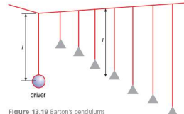
Figure 13.19 Barton's pendulums
