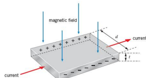
Figure 22.23 The Hall effect
