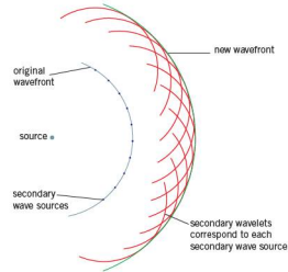
Figure 15.30 Huygens' construction for a circular wavefront
