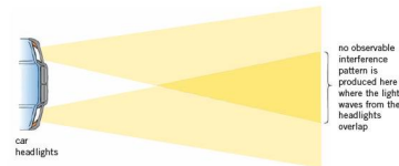
Figure 15.8 Failure of an interference demonstration with light
