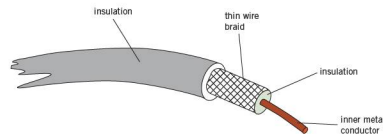
Figure 16.1 Coaxial cable
