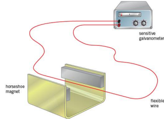
Figure 23.2 Apparatus to demonstrate electromagnetic induction
