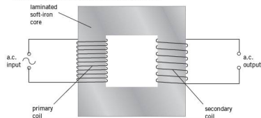
Figure 24.2 Simple transformer
