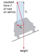
Figure 7.7 Cornering on a banked track
