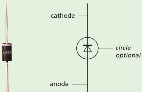
Figure 41.8 A diode and its symbol
