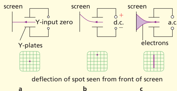
Figure 48.7 Deflection of the electron beam
