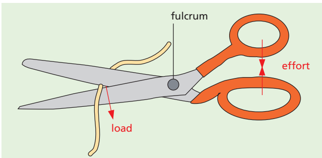
Figure 10.5c Scissors
