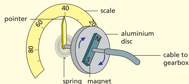
Figure 44.7 Car speedometer
