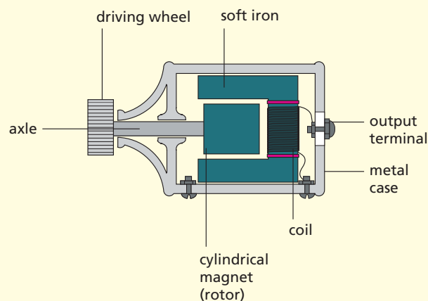
Figure 43.9 Bicycle generator
