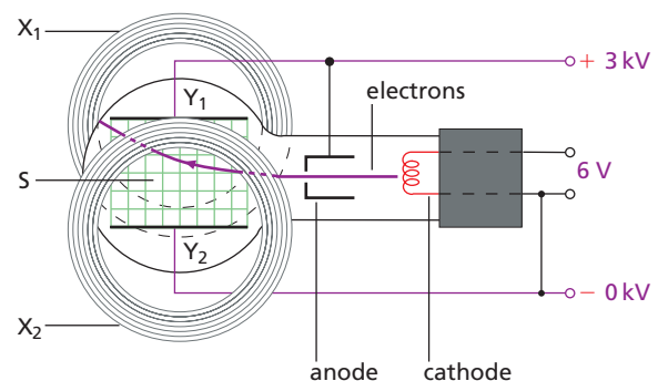
Figure 48.5 Deflection tube
