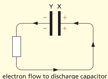
Figure 39.5b Discharging a capacitor
