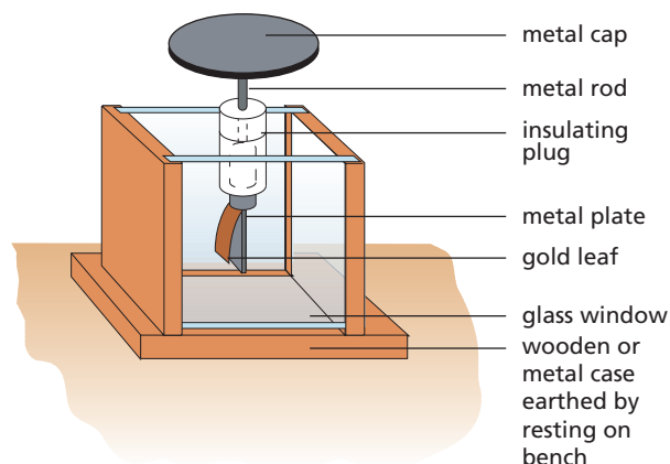
Figure 35.4 Gold-leaf electroscope
