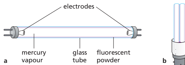
Figure 40.4 Fluorescent lamps
