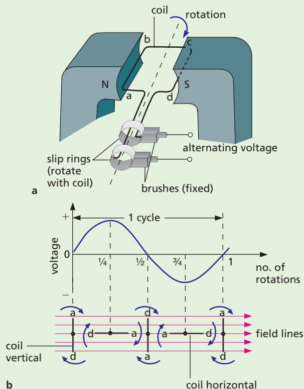
Figure 43.5 A simple a.c. generator and its output
