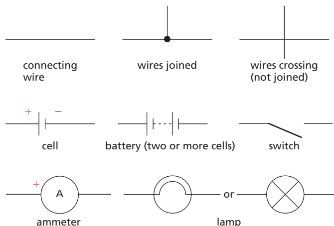
Figure 36.3 Circuit symbols
