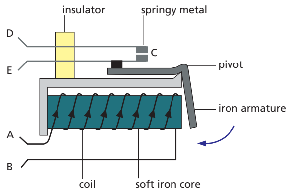
Figure 45.9 Relay
