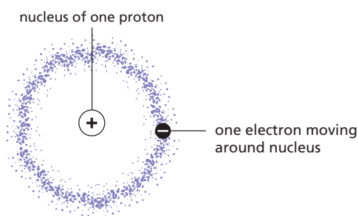
Figure 35.3 Hydrogen atom
