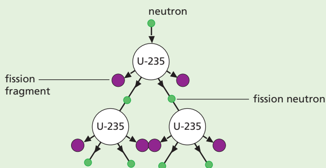
Figure 50.9 Chain reaction
