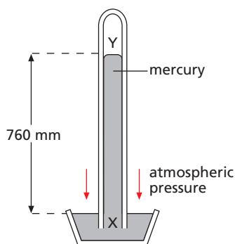
Figure 16.13 Mercury barometer
