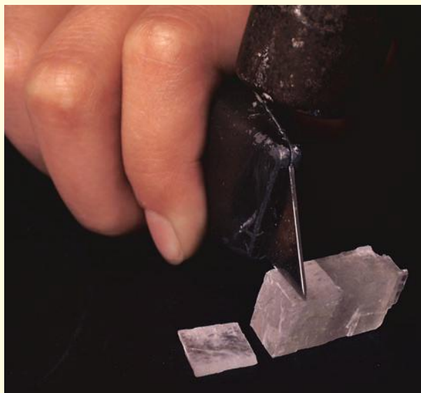
Figure 17.7 Splitting a calcite crystal
