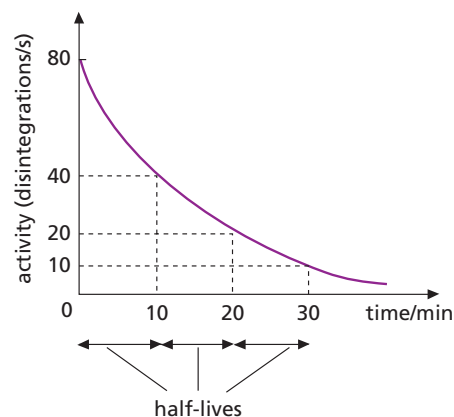
Figure 49.9 Decay curve
