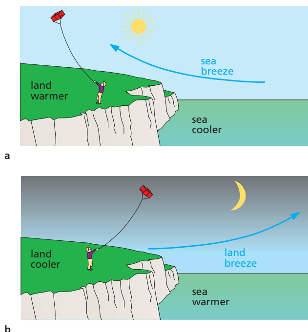
Figure 23.7 Coastal breezes are due to convection: a day; b night
