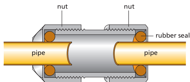
Figure 19.2b Expansion joint
