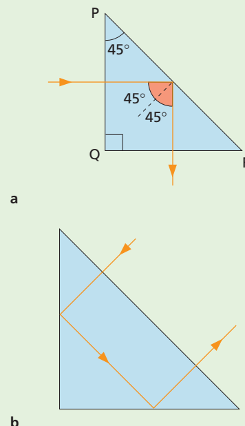
Figure 30.4 Reflection of light by a prism
