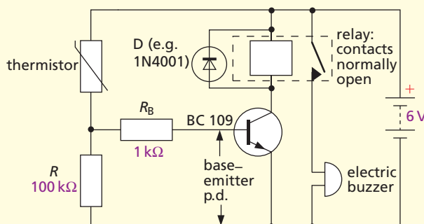
Figure 41.18 High-temperature-operated switch
