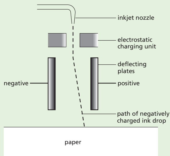
Figure 35.8 Inkjet printer
