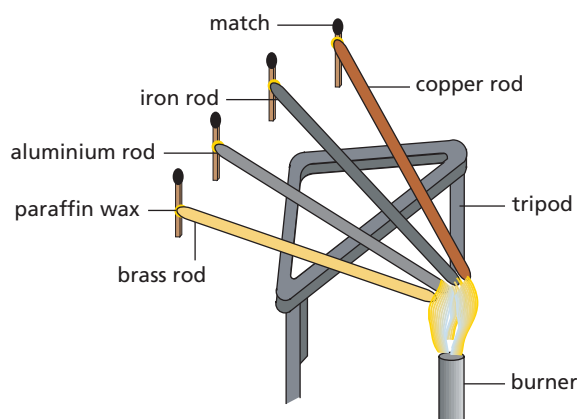
Figure 23.1 Comparing conducting powers
