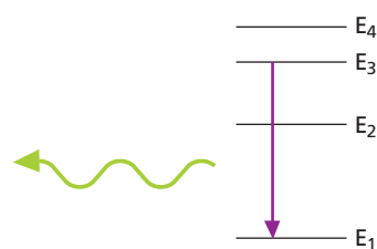
Figure 50.7 Energy levels of an atom
