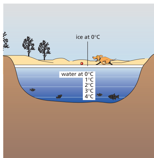
Figure 19.7 Fish can survive in a frozen pond.
