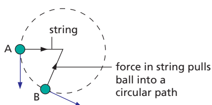
Figure 9.1 ‘Throwing the hammer’
