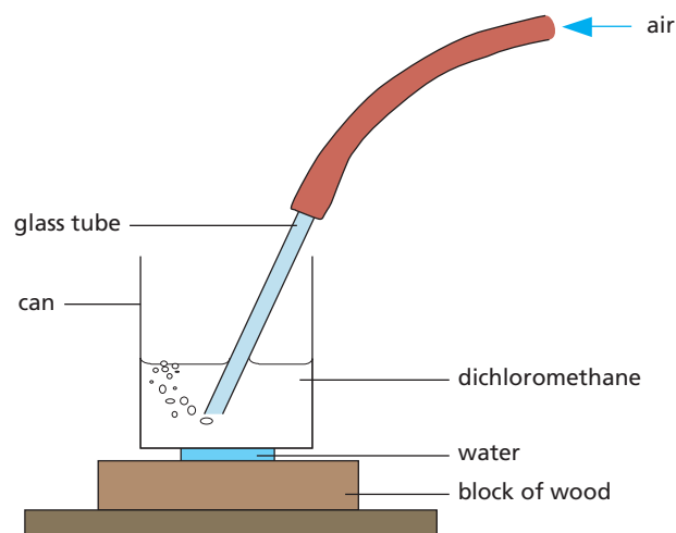
Figure 22.6 Demonstrating cooling by evaporation
