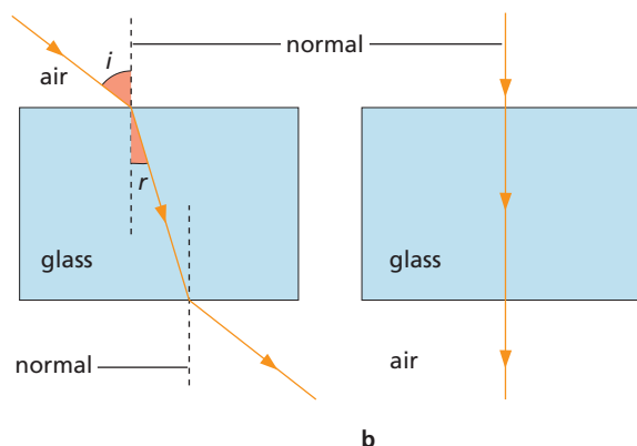
Figure 29.1 Refraction of light in glass
