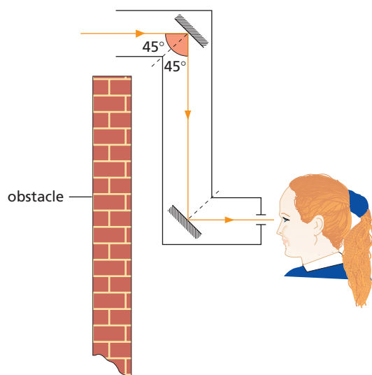
Figure 27.3 Action of a simple periscope
