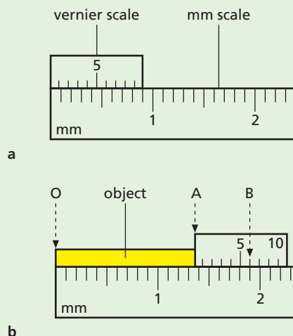
Figure 1.11 Vernier scale
