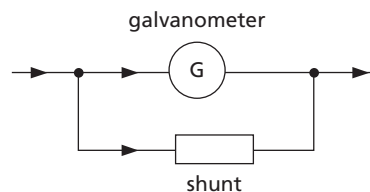
Figure 47.2 An ammeter
