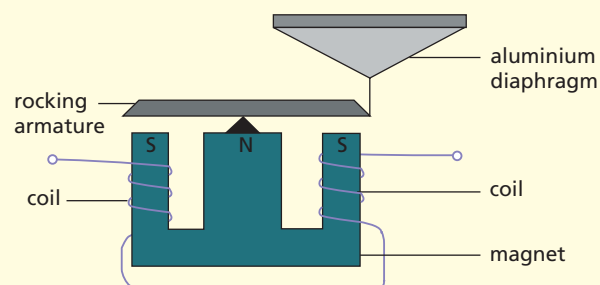
Figure 45.13 Telephone receiver
