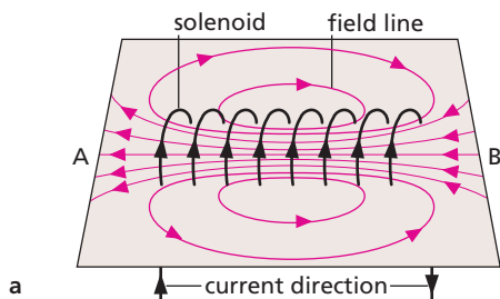
Figure 45.4a Field due to a solenoid
