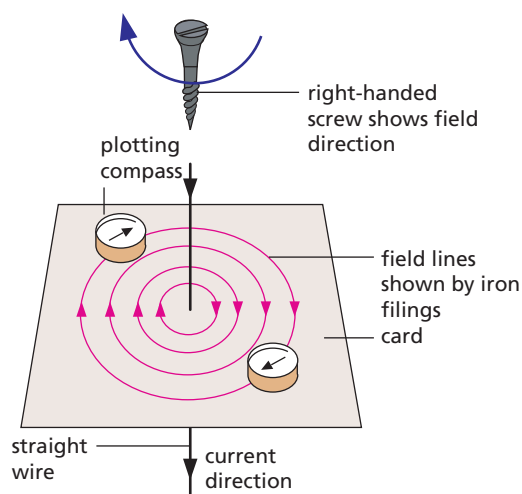
Figure 45.2 Field due to a straight wire
