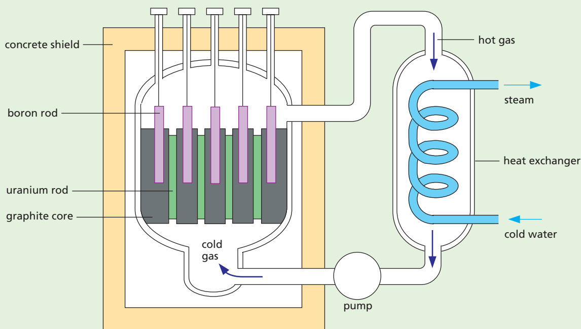
Figure 50.10 Nuclear reactor
