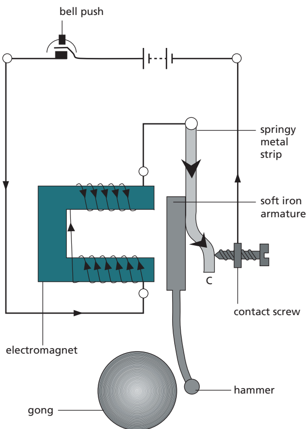
Figure 45.8 Electric bell
