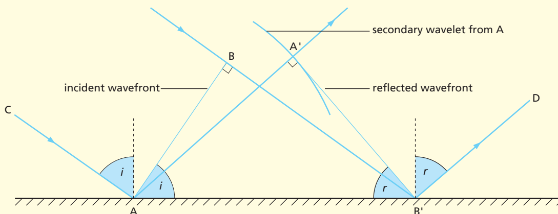
Figure 25.11 Reflection of a straight wavefront
