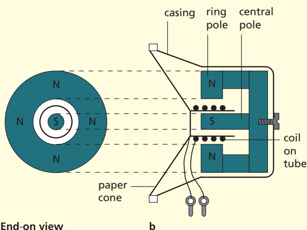
Figure 46.7 Moving-coil loudspeaker
