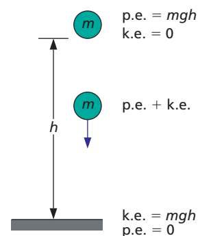
Figure 14.3 Loss of p.e. = gain of k.e.
