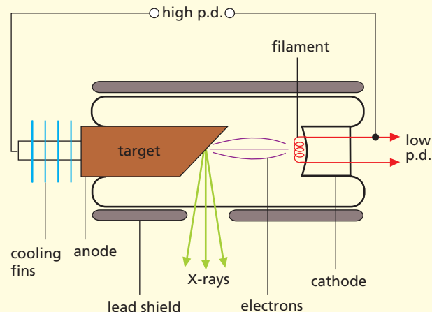
Figure 48.12 X-ray tube
