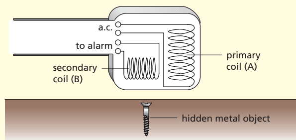
Figure 44.8 Metal detector
