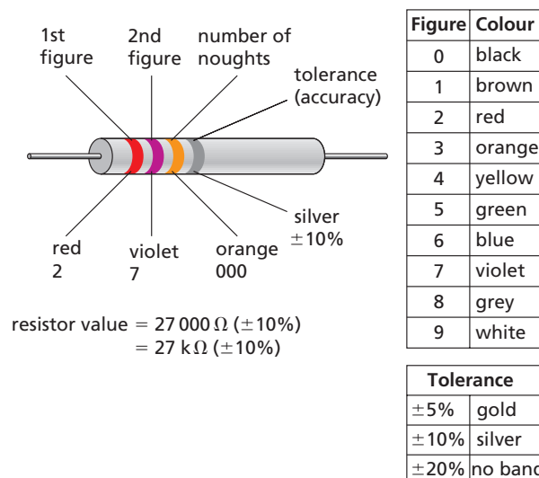
Figure 38.12 Colour code for resistors
