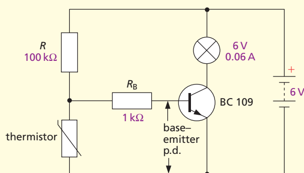
Figure 41.17 Low-temperature-operated switch
