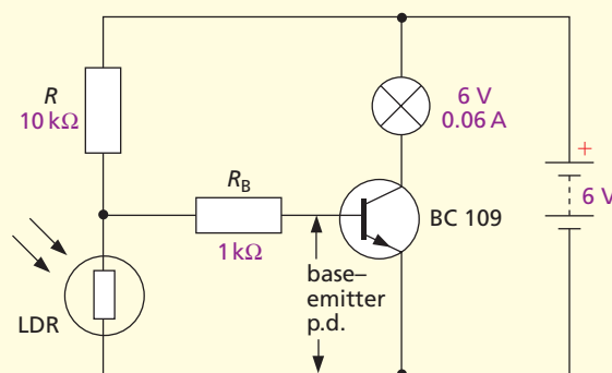
Figure 41.16 Light-operated switch
