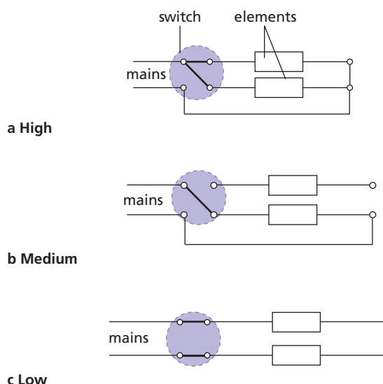
Figure 40.6 Three-heat switch
