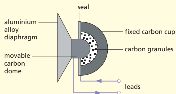
Figure 45.12 Carbon microphone
