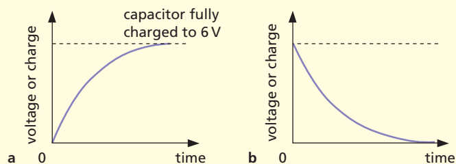
Figure 39.7 Graphs: a charging; b discharging
