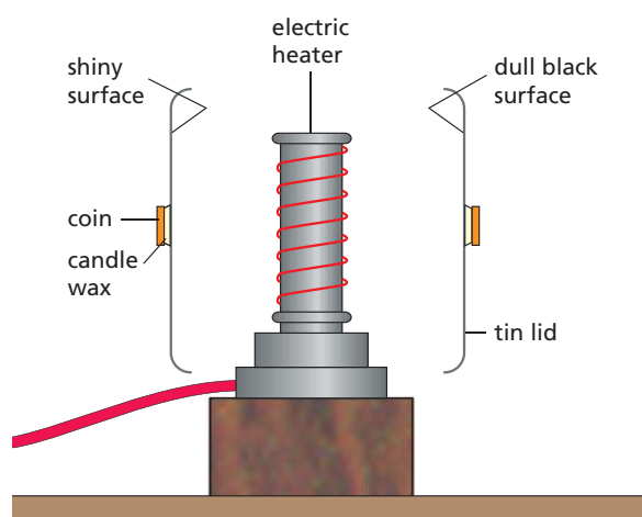
Figure 24.2 Comparing absorbers of radiation
