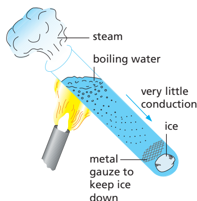
Figure 23.3 Water is a poor conductor of heat.
