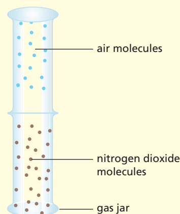
Figure 17.8 Demonstrating diffusion of a gas
