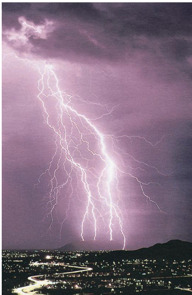
Figure 35.1 A flash of lightning is nature's most spectacular static electricity effect.
