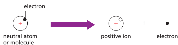
Figure 49.2 Ionisation
