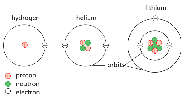
Figure 50.4 Electron orbits
