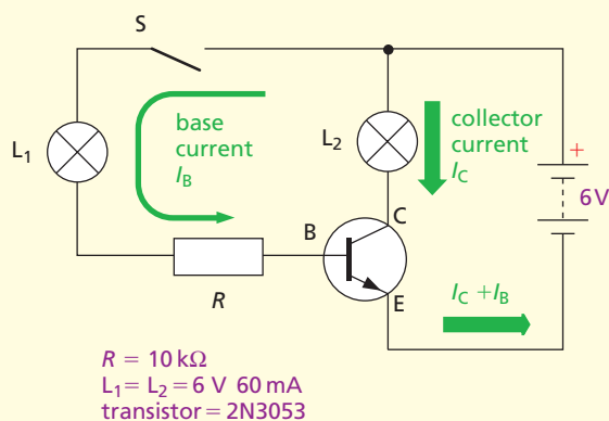
Figure 41.13 Demonstration circuit
