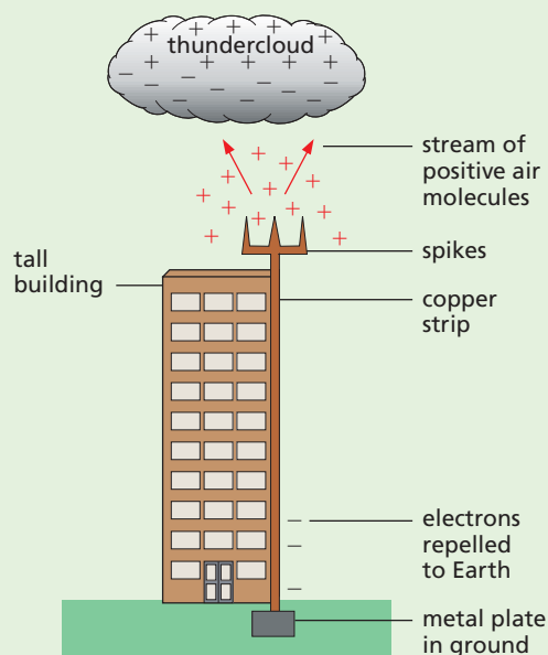
Figure 35.7 Lightning conductor
